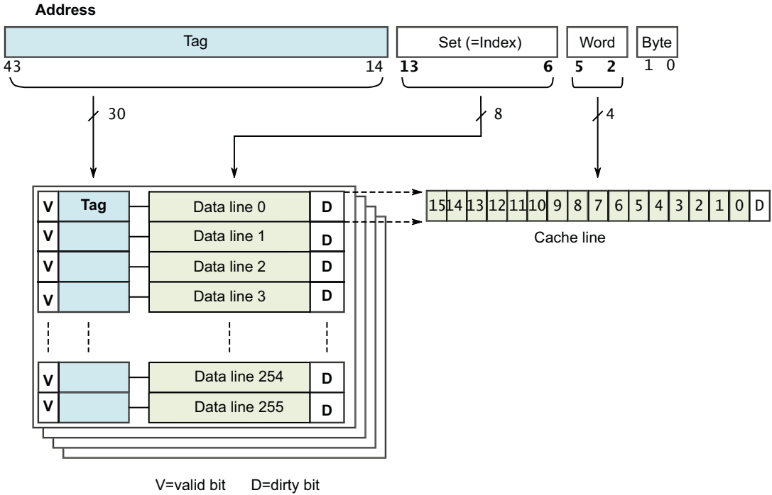
Figure 11-4 A 32KB 4-way set associative data cache
